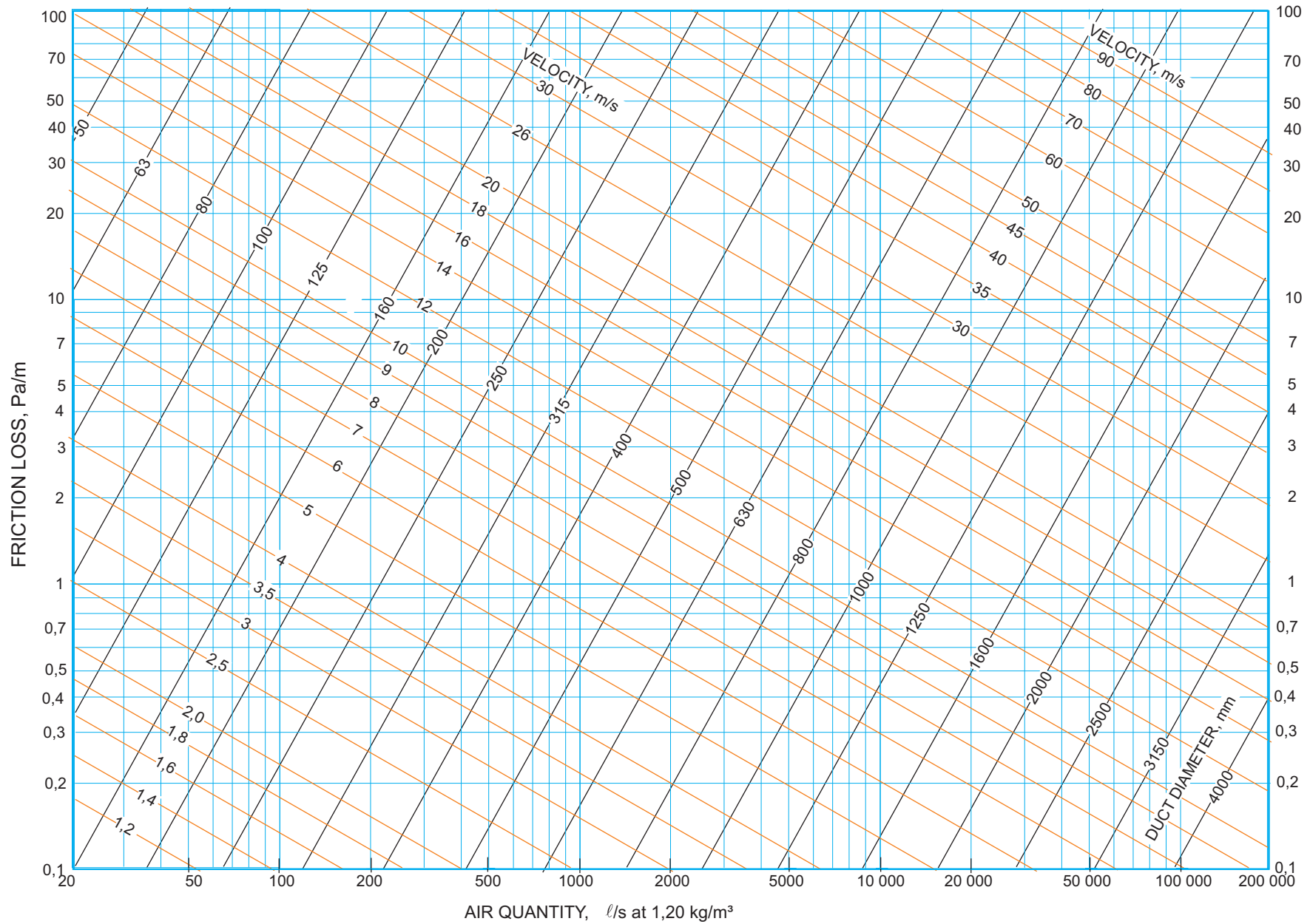
Friction Chart for Round Duct ( \rho = 1,20 \text{ kg/m}^3 and \epsilon = 0,09 \text{ mm} )
