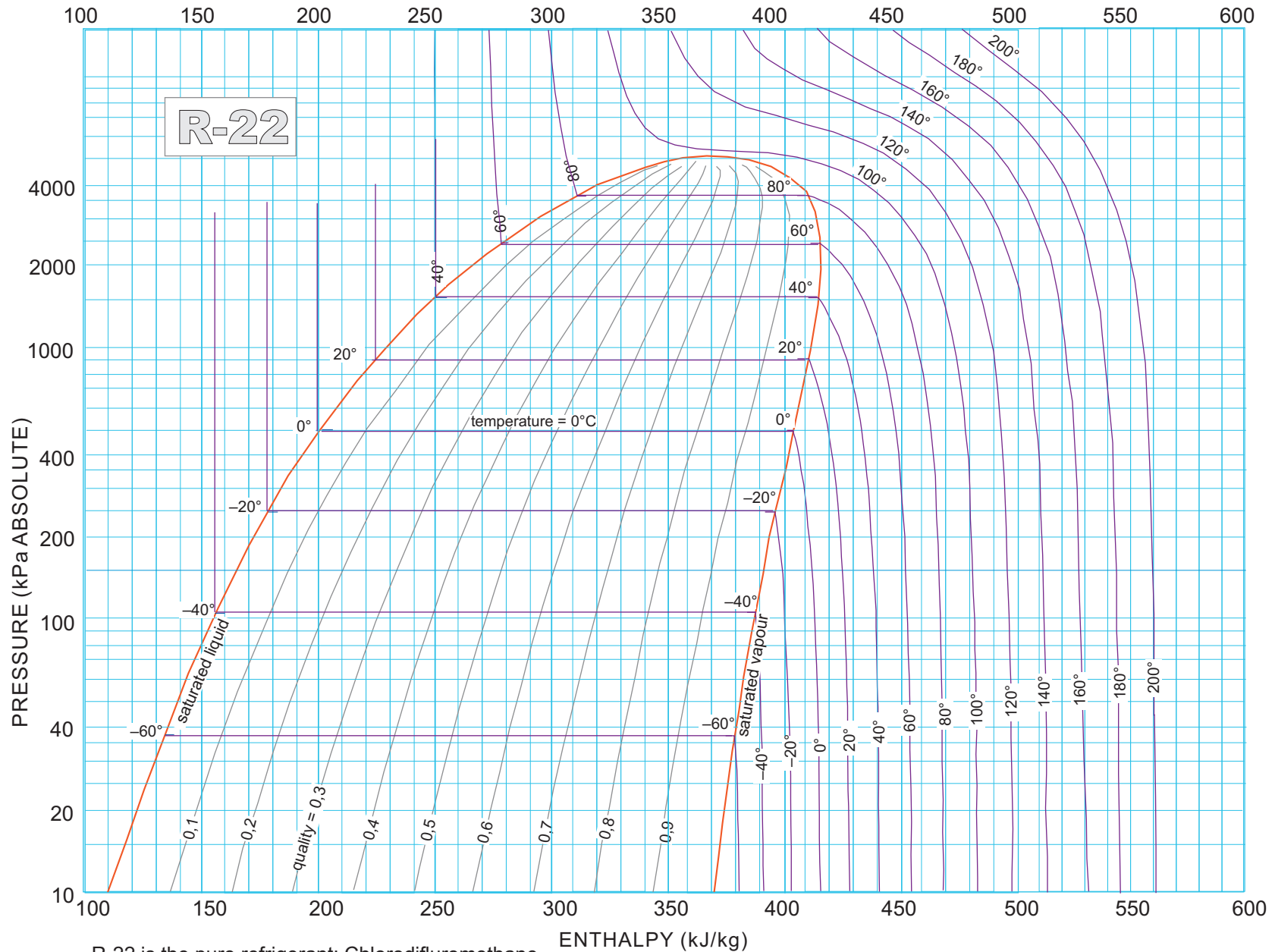
PRESSURE - ENTHALPY DIAGRAM FOR THE REFRIGERANT R-22
