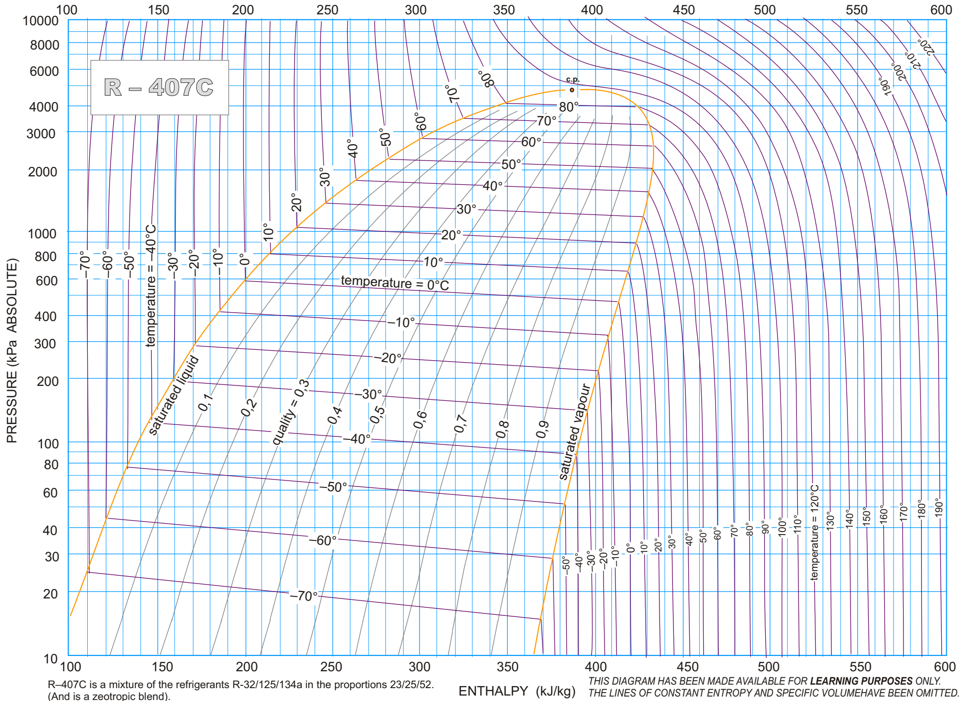
PRESSURE - ENTHALPY DIAGRAM FOR THE REFRIGERANT R-407C
